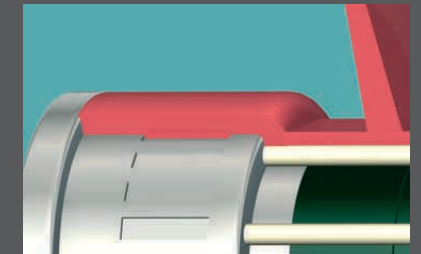
Direct bonding of housing to fittings ensures optimum moisture barrier
